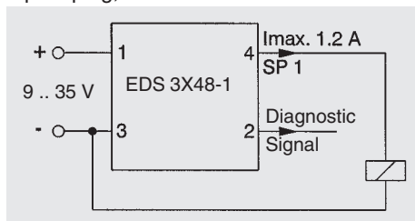
Model which can be connected to DESINA® for self-monitoring: 5 pole plug, M12x1
