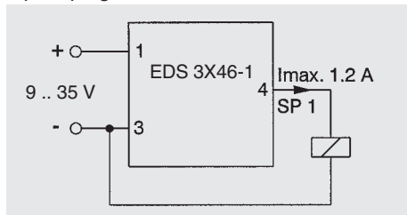
Model with 2 switching outputs: 4 pole plug, M12x1
