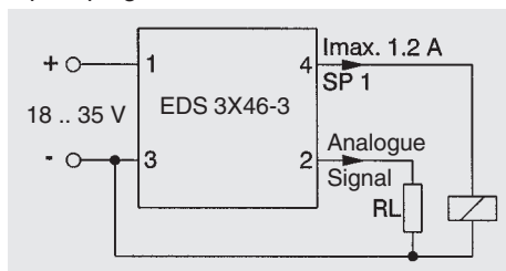
Model with 2 switching outputs and 1 analogue output: 5 pole plug, M12x1
