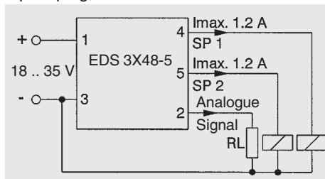
Model to DESINA® standard for self-monitoring: 5 pole plug, M12x1
